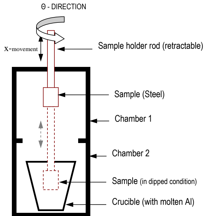
Fig 3: Schematic of sample holding mechanism
