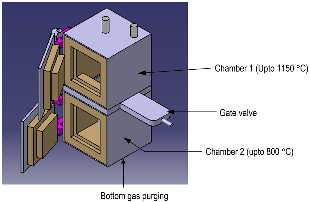
Fig 1: Conceptual drawing of HDA furnace
