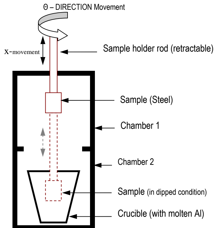
Fig 3: Schematic of sample holding mechanism (Open gate valve condition)
