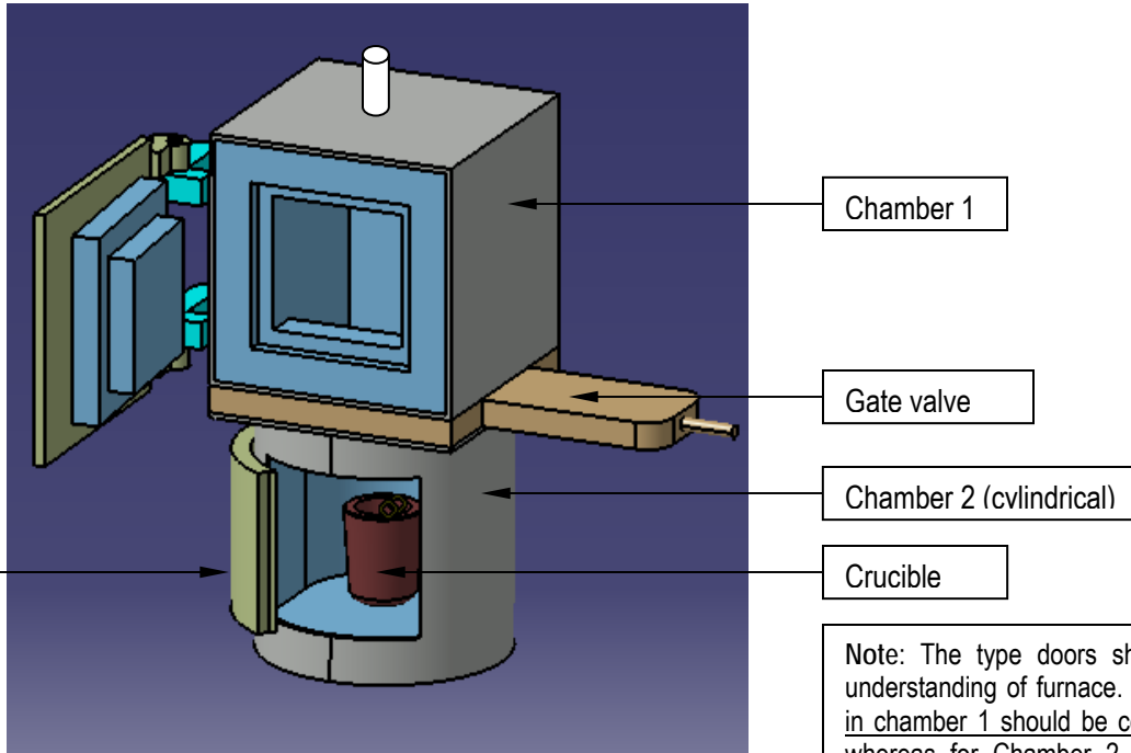
Fig 1: Conceptual drawing of HDA furnace
