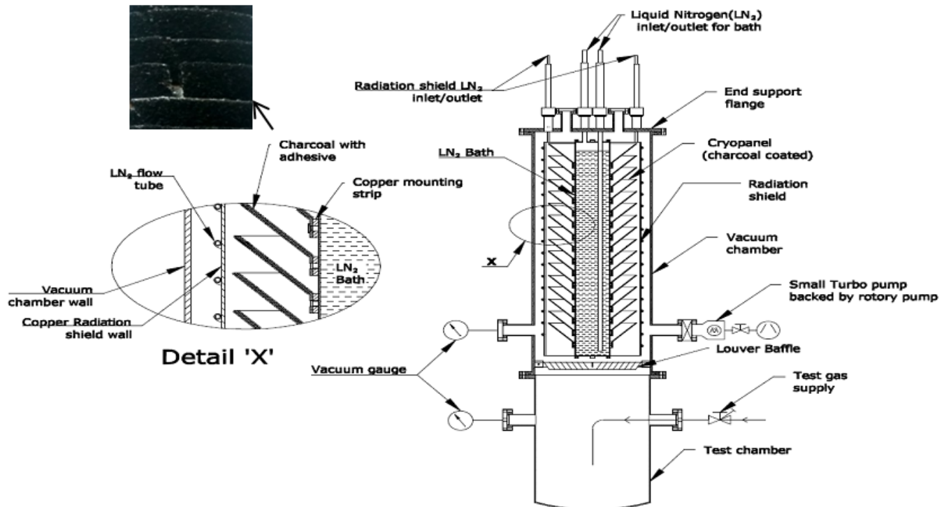
Layout diagram of the CVPS developed by IPR, showing the different components
