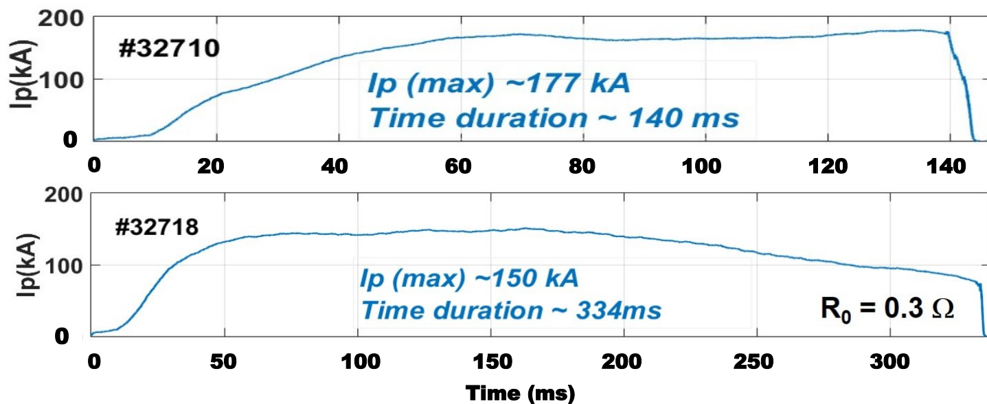
Time evolution of the plasma current from Aditya-U shots
