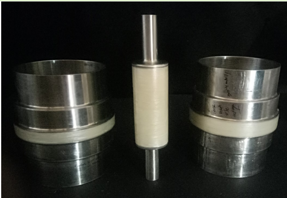
(L) Fully assembled Vacuum Barrier assembly (R) Components of the Vacuum Barrier assembly
