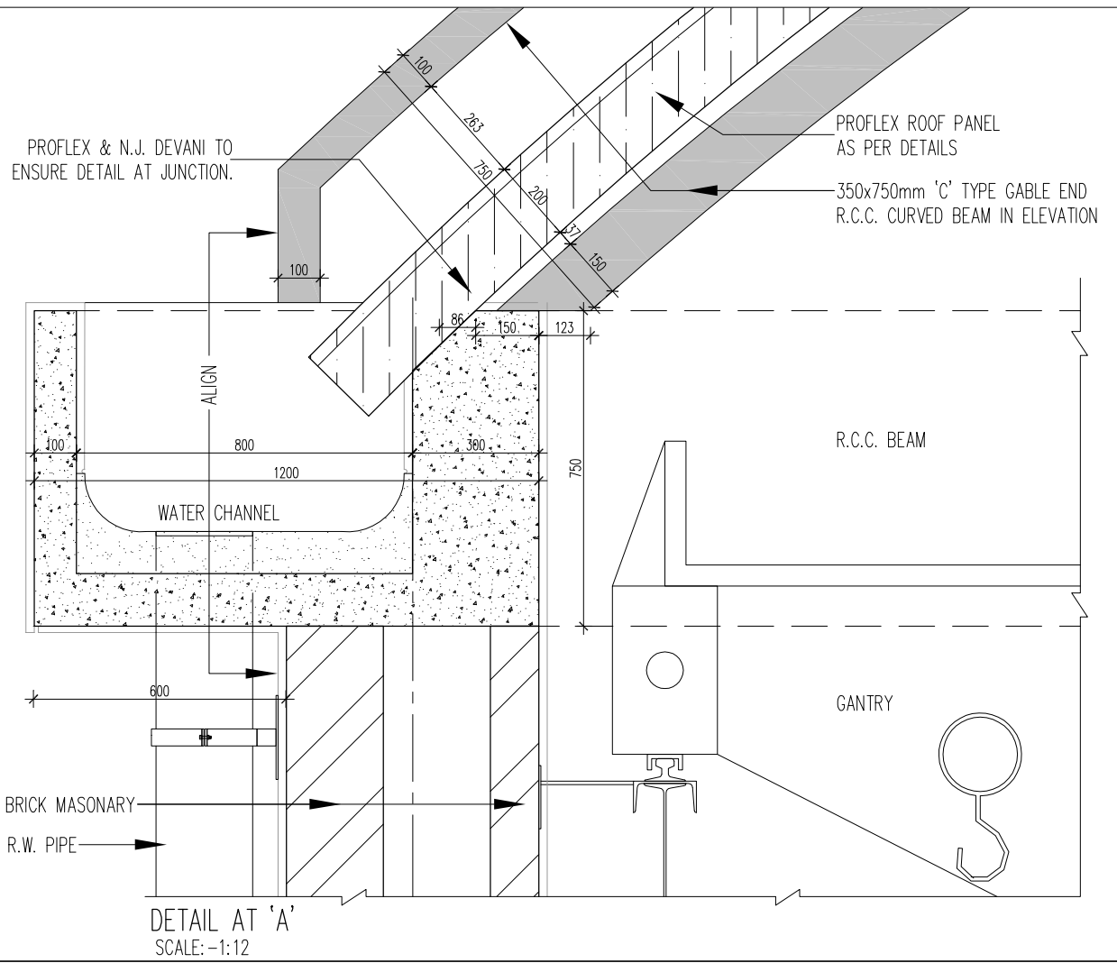
PROFLEX ROOF & R.C.C. BEAM PROFILE DETAILS SCALE: - 1:50
