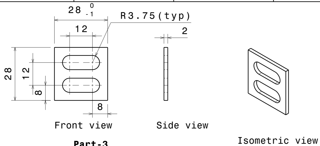
Part-3 Copper plate Material - ETP copper Qty - 2 no.s
