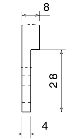
Detail G
