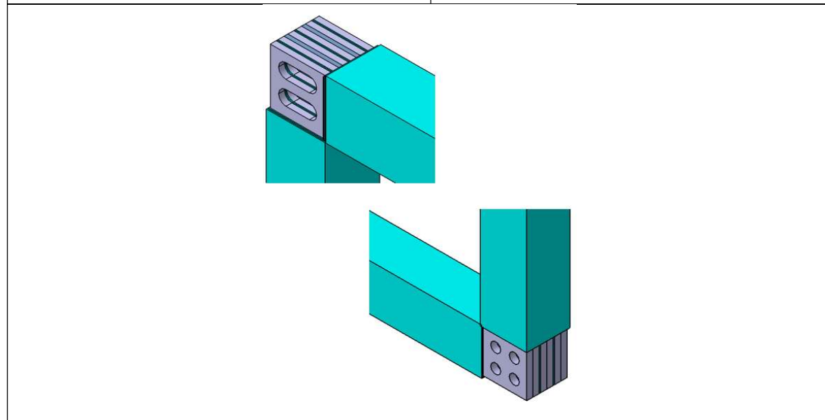
Fig 23. Assembly of Inner & Outer Leg sub-assemblies (top and bottom corner zoomed views) – after inserting copper sheets and Teflon sheets at corresponding locations
