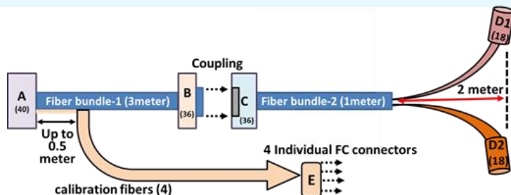
(L) XRCS-Survey Spectrometer integrated in Equatorial Port -11 (R) Schematic of the optical fiber bundle Assembly with all the required terminations and bundle to bundle coupling.
