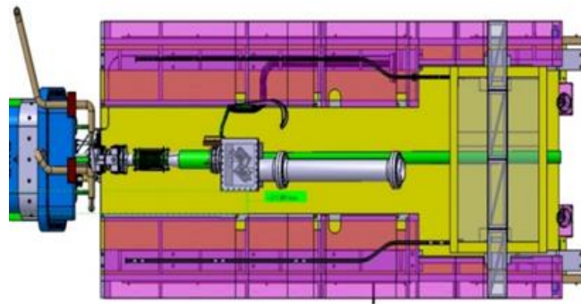
(L) Overview of ECE Diagnostic (R) XRCS-Edge spectrometer integrated in Upper Port -9
