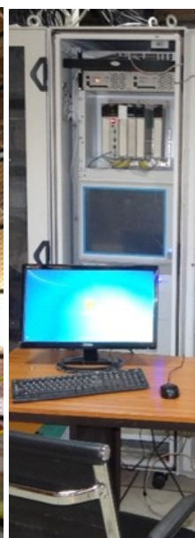
100kV, 25 A Regulated High Voltage Power Supplies (RHVPSs) installed at BARC site. Waveform shows 80kV application by RHVPS at repetition rate of 2Hz to Klystron cathode
