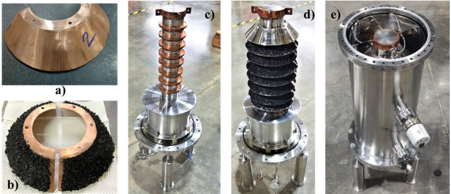
(a) Bare copper panel half (b) Pair of charcoal coated panel (c) SS bath and copper collar rings, (d) charcoal coated panels assembly and assembled cryopump (kept inverted)
