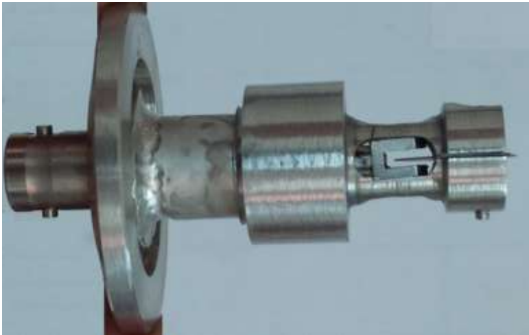
(L) The miniature Penning Ionization Gauge (R) The gauge being tested on an experimental stand.
