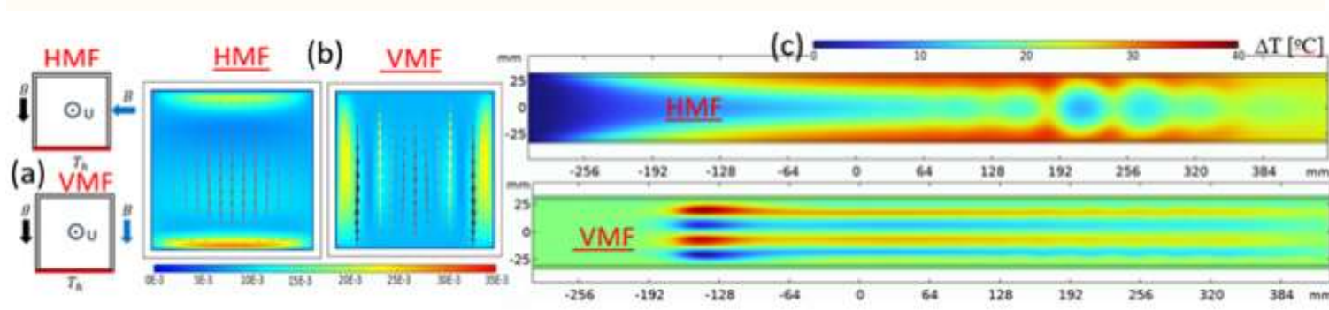
Figure: (a) Heating configuration in square duct for HMF & VMF, (b) comparison of velocity ( U [m/s]) profile in HMF and VMF cases at 10 mm away from the heated section, (c) comparison of temperature distribution in the mid horizontal plane
