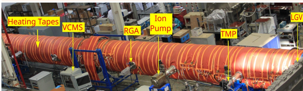
Integrated Vacuum Vessel (IVV) post assembly
