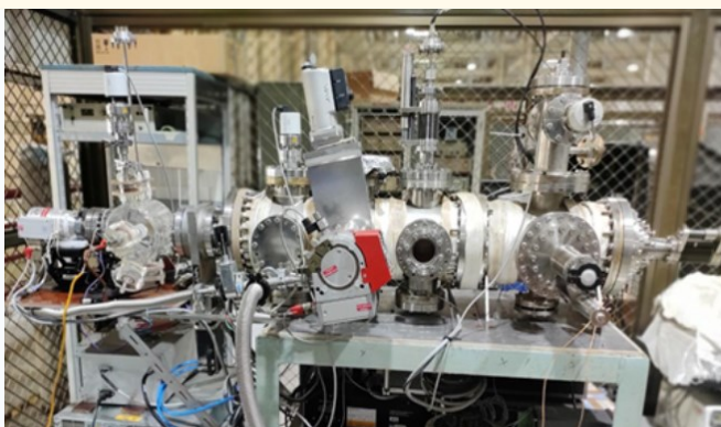
Indigenously developed SMBI System
