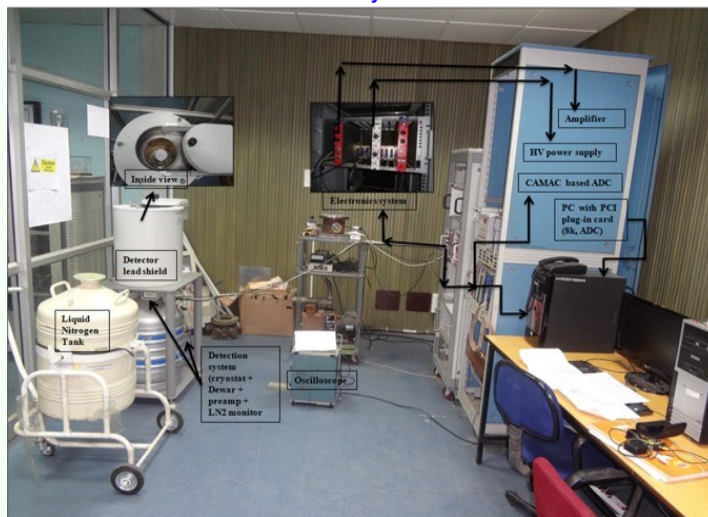
Fig. 3 Experimental set-up of off-line gamma ray spectroscopy
