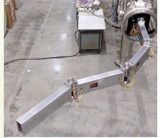
In-vessel Inspection System (IVIS)
