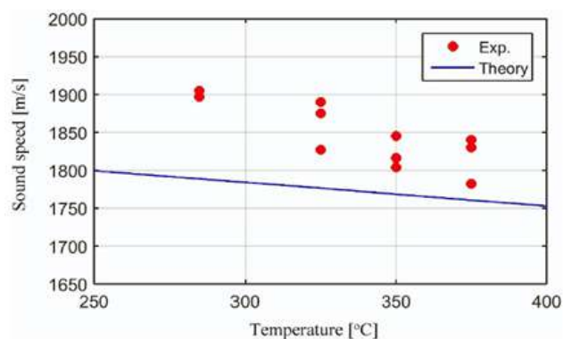
Figure A.4.9: Variation of sonic velocity of Pb-Li with temperature.
