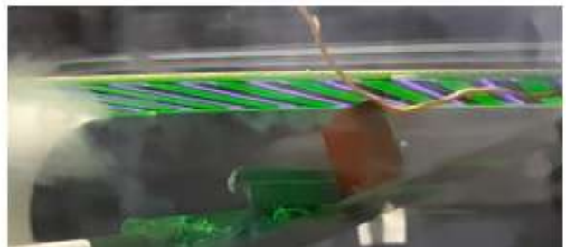
Figure A.1.22: Smoke visualization of surface flow over an aerofoil without and with plasma.
