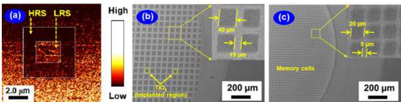
Figure A.1.14: (a) Demonstration of two-fold erase-write process. Field emission scanning electron microscopy image of a periodic array of \text{TiO}_x -based squared memory cells of different sizes fabricated by plasma fireball using masking method. Memory size (b) 40 \mu\text{m} and (c) 20 \mu\text{m} .
