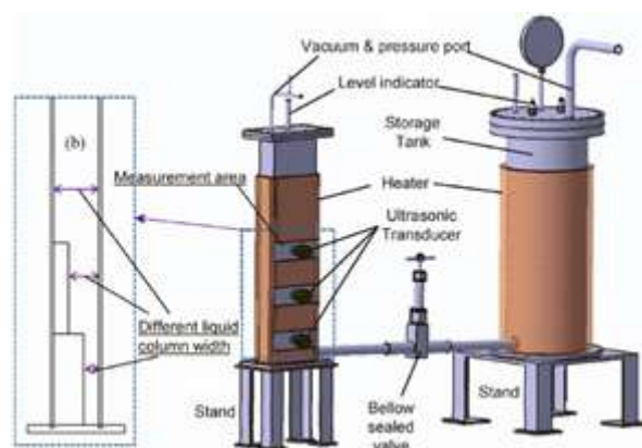
Figure A.4.8: Experimental set up for sonic velocity measurement of fluids at high temperature.
