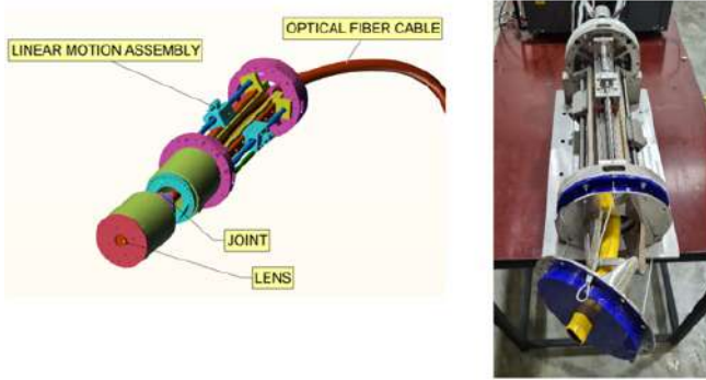
Figure A.4.16: Prototype manipulator for maneuvering the lens bundle.
