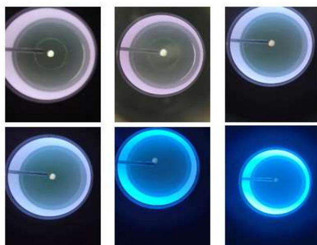
Figure A.2.19: Hairpin probe inserted radially in oxygen plasma. The bright regions at the edge shows the high energy electron population while the core is dominated by negative ions.
