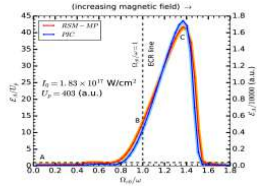
Figure A.5.9: Average absorbed energy per electron \mathcal{EA} vs its normalized cyclotron frequency \Omega c_0 from a laser-driven deuterium nano-cluster with increasing external magnetic field. Absorption is less than U_p for negligible external magnetic field (at point A) while it is 12U_p and 43U_p at points B (for ECR, electron cyclotron resonance) and C respectively.
