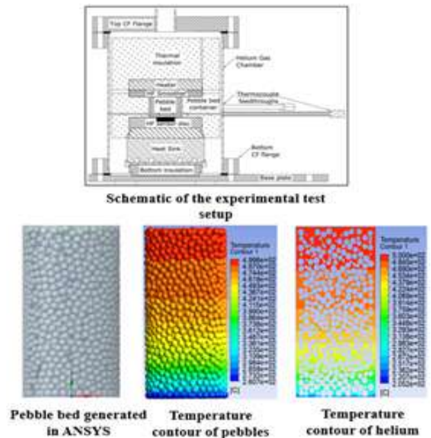
Figure A.5.10: Schematic of experimental test setup and simulation data.
