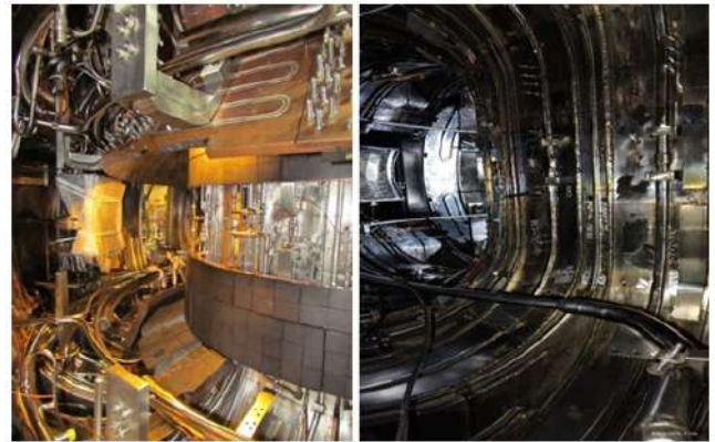
Figure A.3.8: Inside view of SST-1 vacuum vessel before and after PFCs removal.
