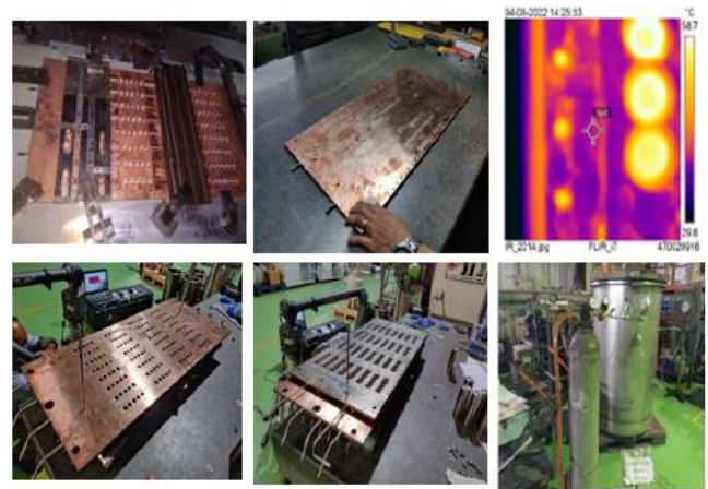
Figure A.4.19: Development of the grid system for the TWIN source using brazing.
