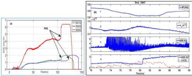
Figure A.3.17: (a) Steep Rise in ECE amplitude signifying the PAS events (b) temporal evolution of: (1) plasma current (IP), (2) density ( n_e ), (3) Hard X-Rays (HXR) and (4) Loop Voltage (LV) & ECE amplitude.
