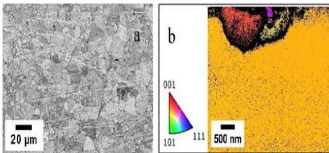
Figure A.4.2: FESM micrograph (a) shows the grain structures on the plasma exposed surface of WP1 (1866K), EBSD IPF map of the FIB made crosssection of WP1 (b) shows small grains along the exposed surface which still remains deformed.
