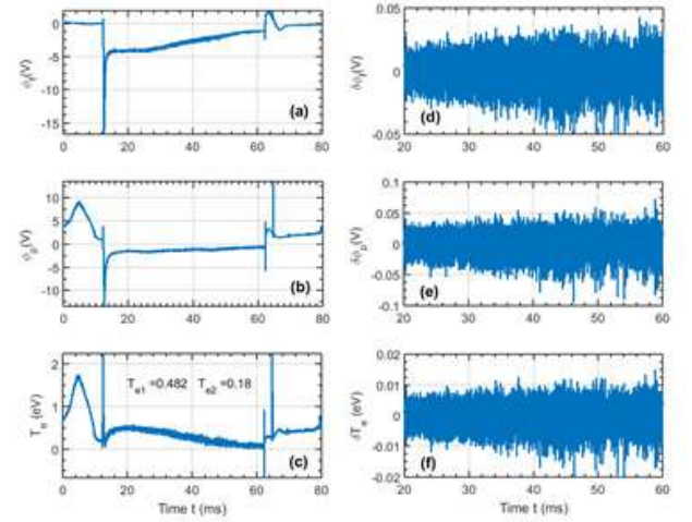
Figure A.2.3: This shows simultaneous measurement of a) floating potential, b) plasma potential, c) electron temperature and their respective fluctuations.
