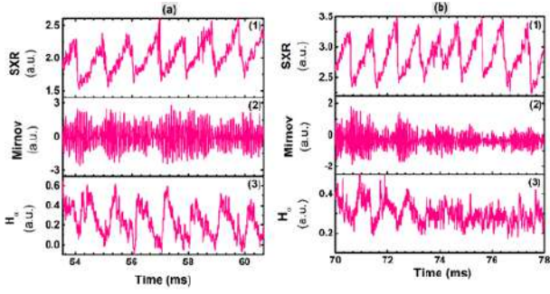
Figure A.3.1: Sawtooth in SXR and H_\alpha signal for different amplitude of Mirnov oscillations, (a) relatively strong MHD (shot#13262&14139) (b) relatively weak MHD (shot#14176).
