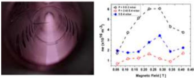
Figure A.2.16: The above figure shows a col-limated argon plasma produced in APPEL at a magnetic field strength of 0.4T and a background pressure of 2 \times 10^{-4} mbar. The experiment demonstrates the possibility to produce plasma at low pressures with ionization efficiency typically less than 5 % using the helical plasma device provided the magnetic field lines are normal to the plane of the antenna.
