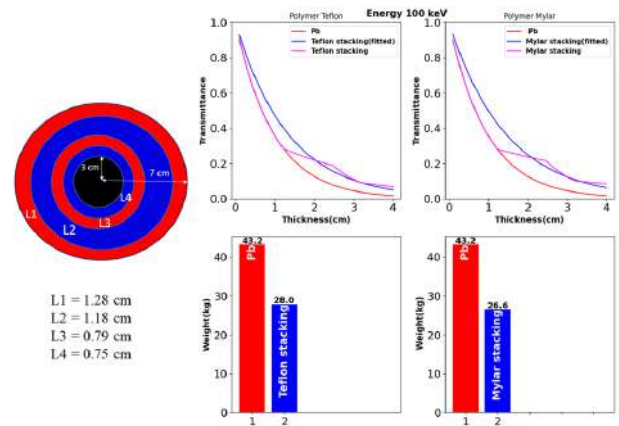
Figure A.3.16: Schematic of proposed shield along with study of transmittance with shield length and reduction in weight using composite of polymer and lead.
