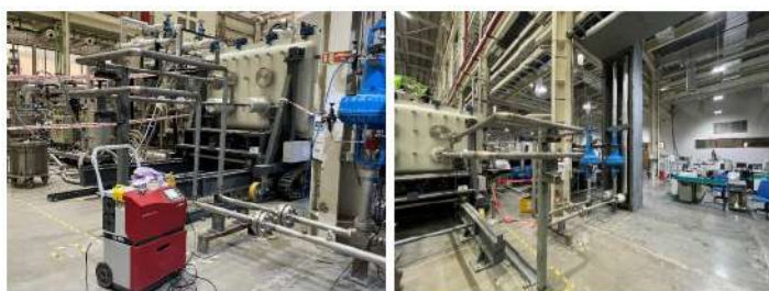
Figure A.2.3: Piping connection between High Heat Flux Test Facility (HHFTF) and Experimental Helium Cooling Loop (EHCL) has been completed. Thermal insulation of the entire piping connections (not shown above) is also completed.
