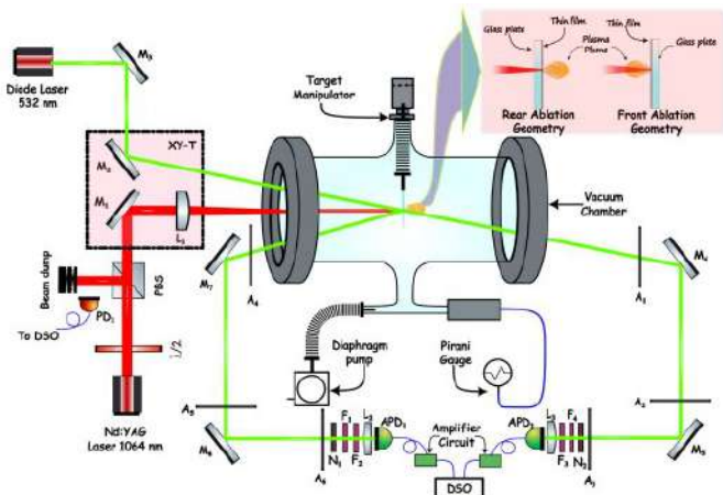
Figure A.1.23: Experimental pump-probe setup for measuring transmittance and reflectance. M-Mirror, A-Aperture, L-Lens, N-Neutral density filter. F-interference filter, APD- Avalanche photodiode, PBS -Polarizing beam splitter, PD-Photodiode, -Half wave plate, XY-T-Automated XY translation stage, DSO-Digital Storage Oscilloscope.
