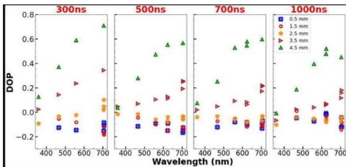
Figure A.I.24: Variation of DOP with emission wavelength at different times after the laser ablation. Different points represents various locations within the plasma. The maximum error in the estimated DOP is expected to be around 10 %.
