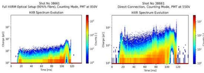
Figure A.1.32: Time and energy resolved count rate registered by the HXR systems during a plasma discharge #38661 with the prototype ITER HXR as shown in the left plot and results obtained using conventional HXR configuration are shown in the right side plot.
