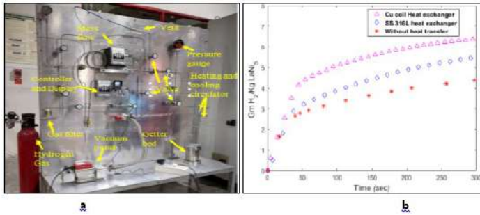
Figure A.2.18. (a) A photograph of Getter bed system for hydrogen isotope storage (b) Hydrogen absorption evolution for \text{LaNi}_5 with and without heat transfer.
