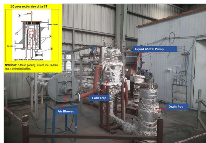
Figure A.2.10: Pb-16Li purification loop . Schematic of CT internal flow configuration is shown at the top corner.
