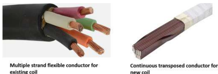
Figure A.1.7: Comparison of conductor configuration for the existing and new poloidal field coils winding.
