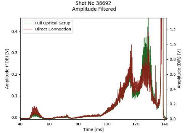
Figure A.1.33: The output signals of the PMTs operated in the current mode operation shows the waveform for the channel working in the direct connection (conventional HXR) and for the channel working with the full optical setup (prototype ITER-HXR) is consistent and comparable.
