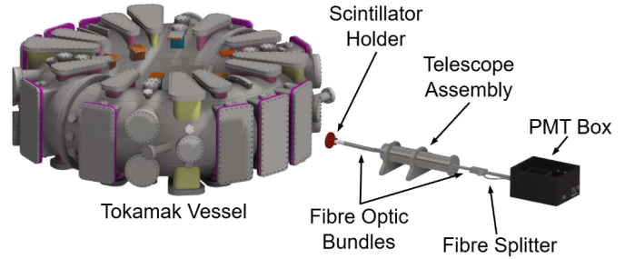
Figure A.1.30: Visualisation of the ADITYA-U tokamak with the ITER HXR prototype components at its installation location just outside the tokamak.
