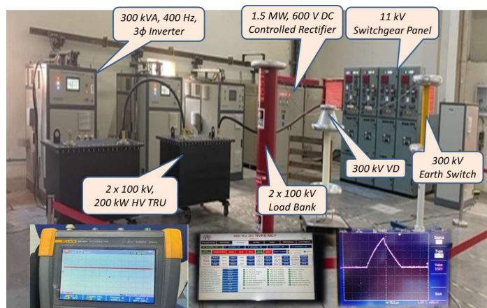
Figure A.6.2: Development of 300kV, 2A DC power supply.
