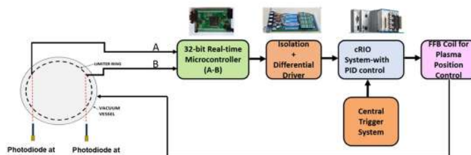
Figure A.1.8: Interconnection of various systems for horizontal plasma position control in ADITYA-U.
