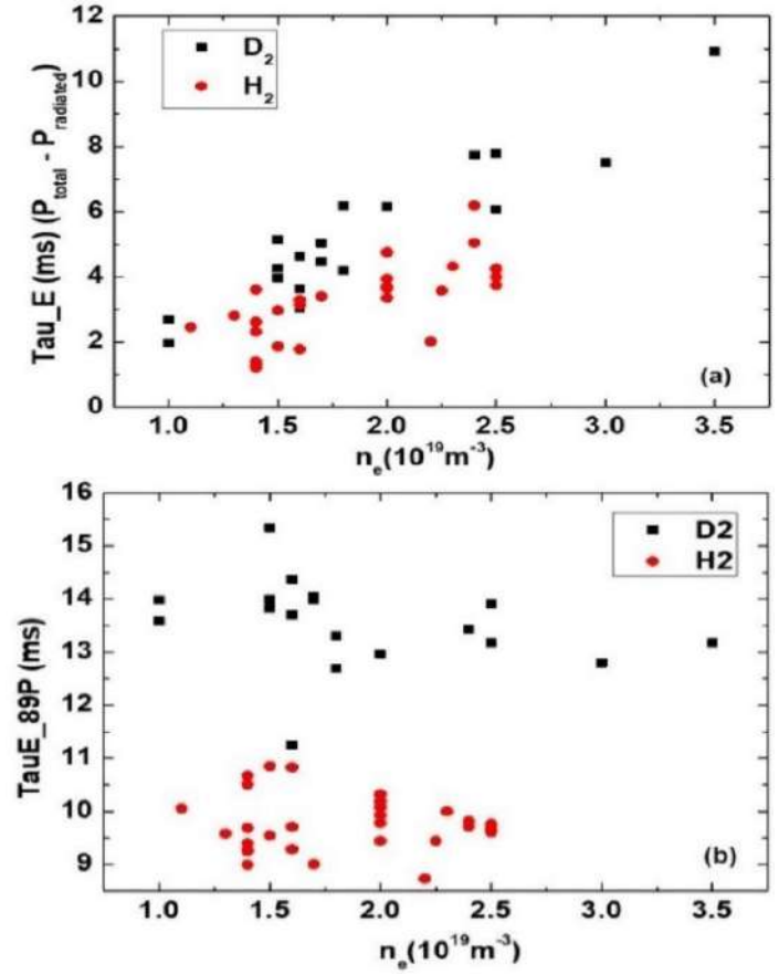
Figure A.1.2: The \tau_E scaling related to line average density for \text{H}_2 and \text{D}_2 Ohmic discharges in ADITYA-U: (a) \tau_E experimental, and (b) \tau_E according to ITER-89P L-mode confinement scaling law.
