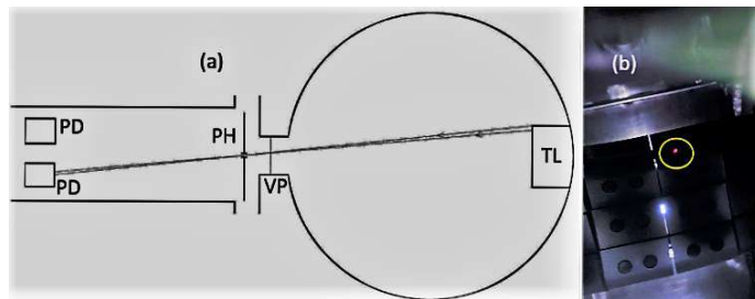
Figure A.1.4: Schematic ray diagram of detector system (a). Deciding location of interest for light collection by back-lighting the pin-hole (b).
